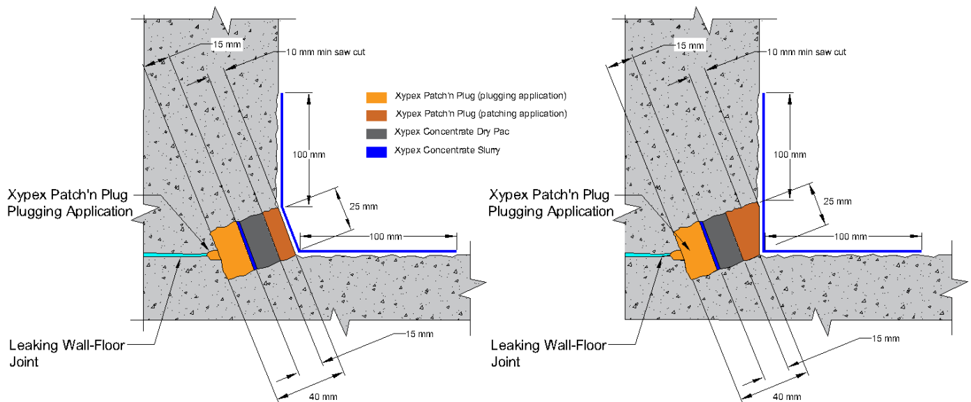
Figure 2, Details of the leaking wall-floor joint repair/cold joint (Schematic)
