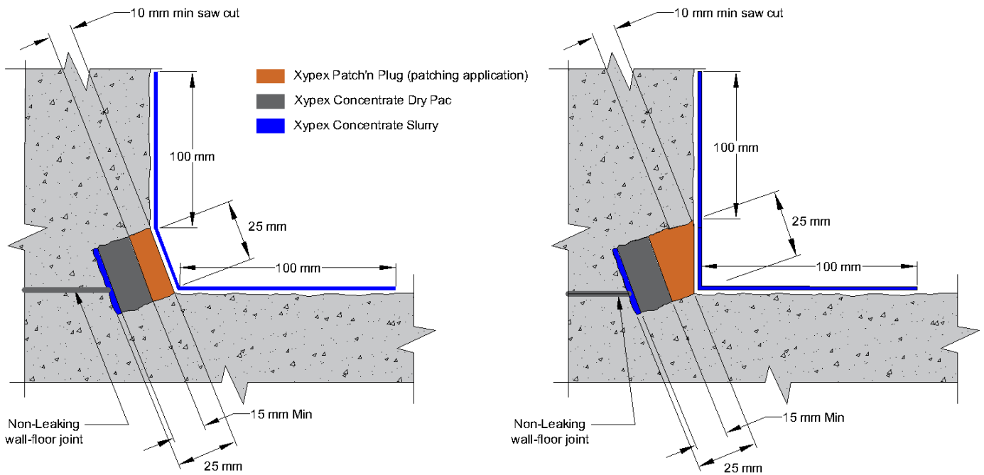
Figure 4, Details of the non-leaking wall-floor joint repair (Schematic)
