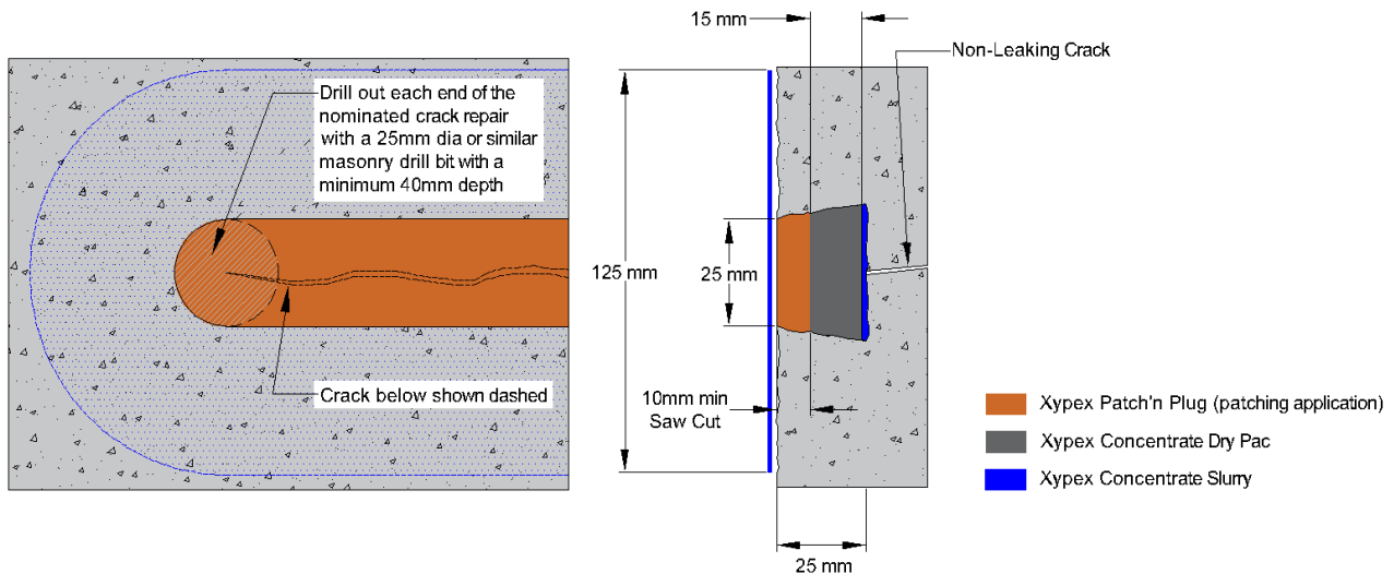
Figure 3, Details of the non-leaking crack repair/cold joint (Schematic)
