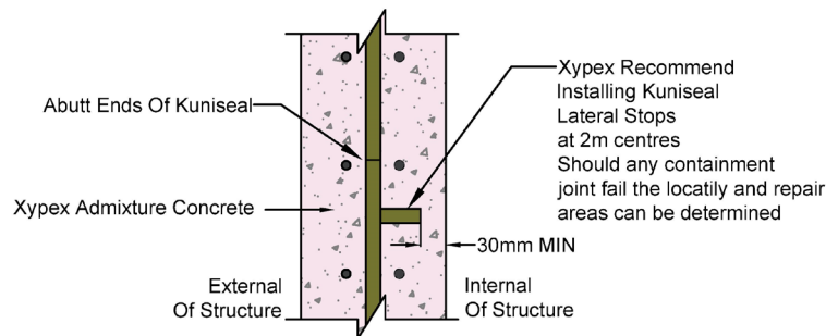
Plan View - Kuniseal Installation
