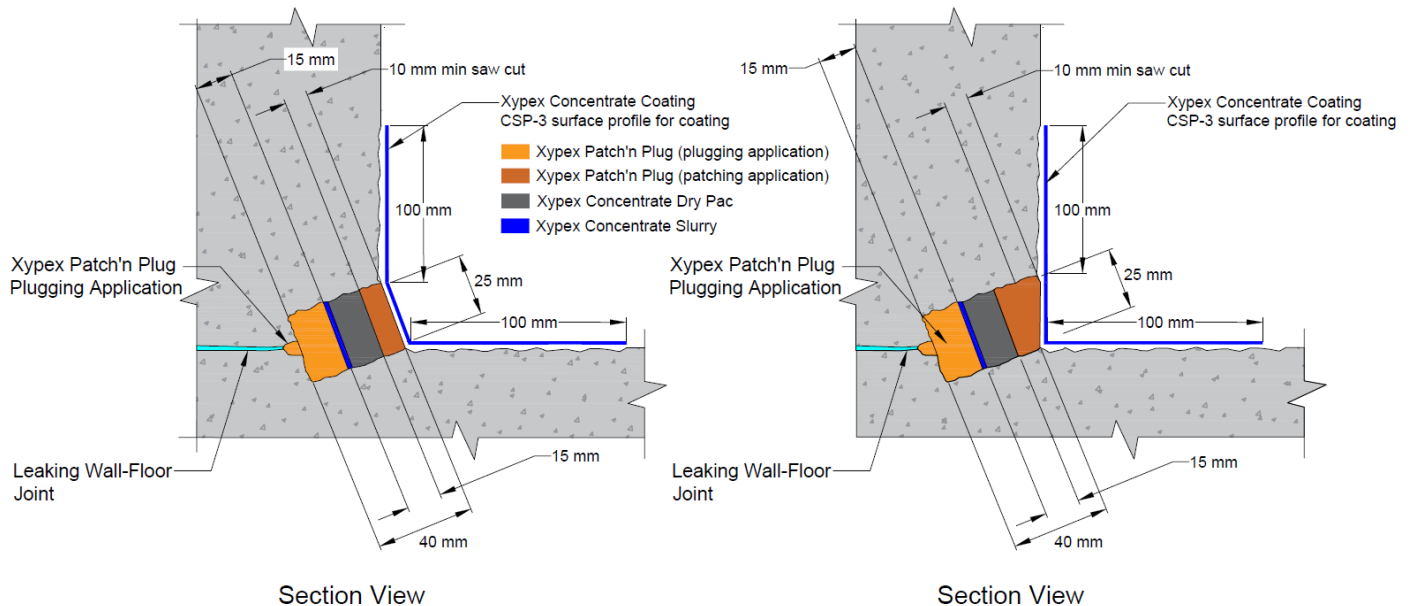
Figure 2, Details of the leaking wall-floor joint repair/cold joint (Schematic)
